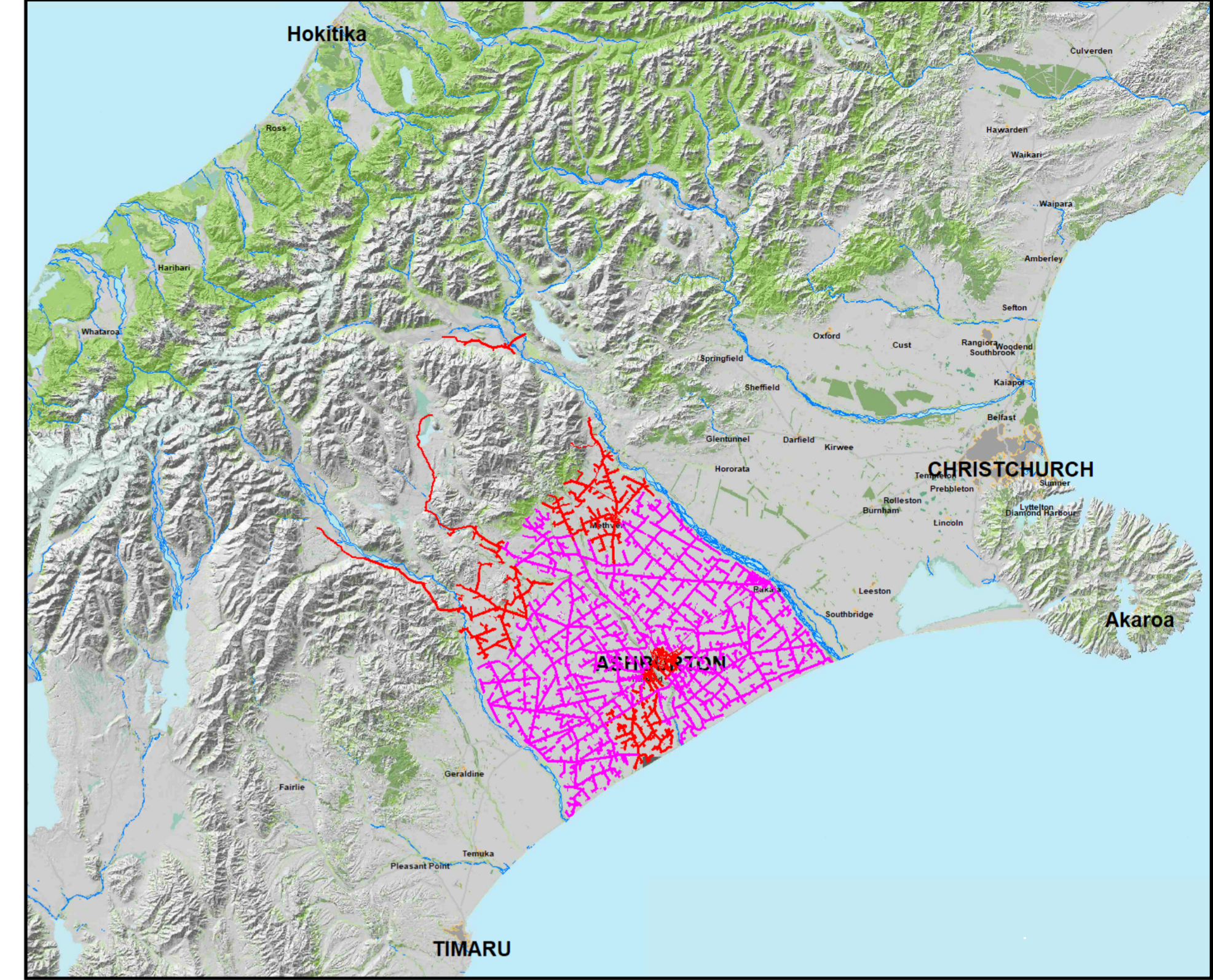
Inset showing EA Networks' location in New Zealand context and 22kV (magenta) and 11kV (red) distribution network. (OA), (OB), (OD), (OF), (OI), (A), (C), (E), & (G)
